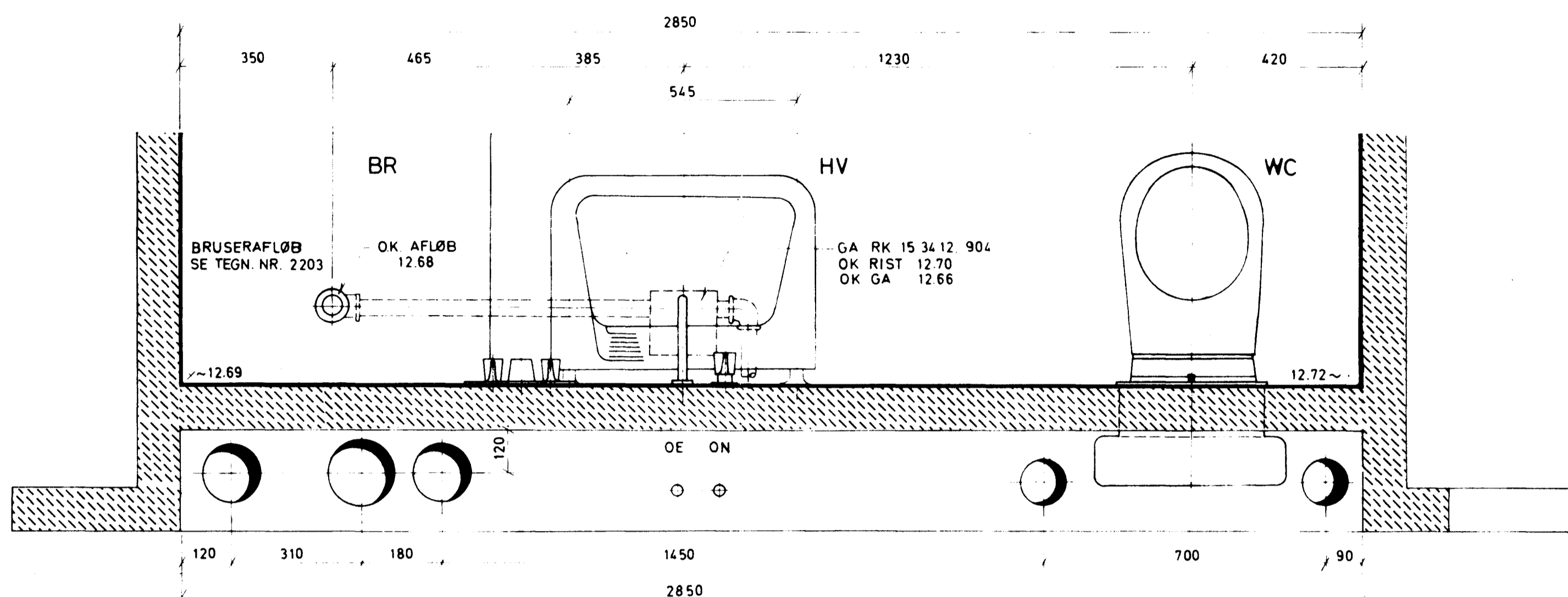
SNIT C-C, PLAN - OVERETAGE.
